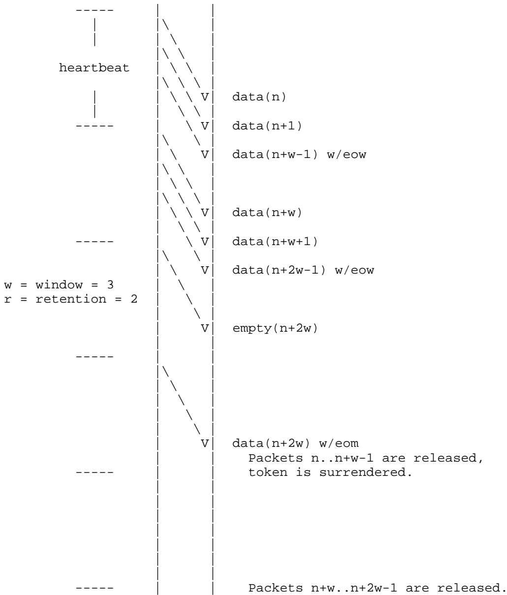
Figure 6. Normal data transmission
