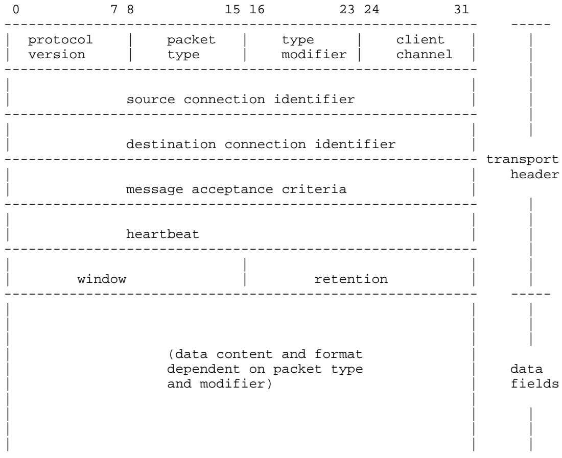
Figure 1. MTP packet format
