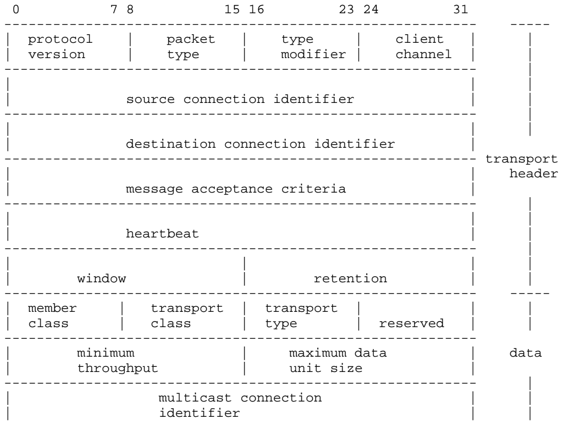
Figure 3. join packet
