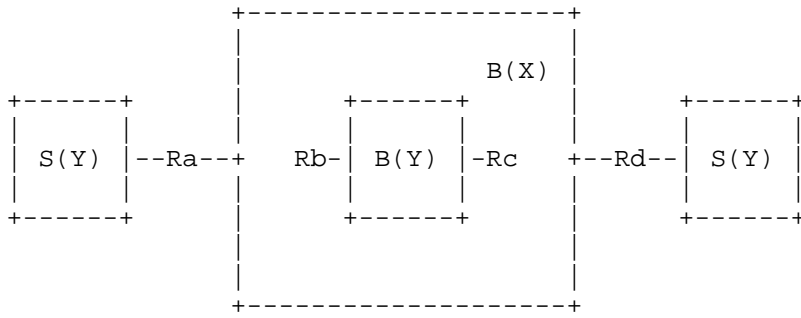
FIGURE 2: NESTED MUTUAL ENCAPSULATION
