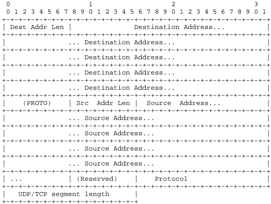
Figure 6-1. Pseudo-header
