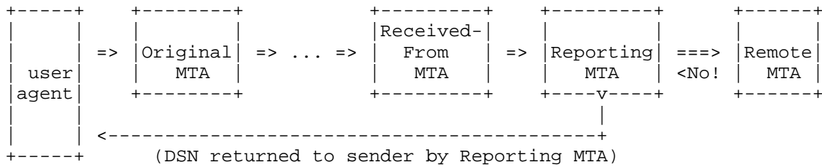
Figure 1. Original, Received-From, Reporting and Remote MTAs
