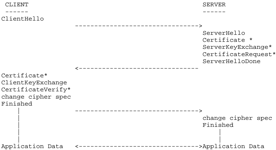
FIGURE 1: The TLS protocol. All messages followed by a star are optional. Note: This figure was taken from an IETF document [1].
