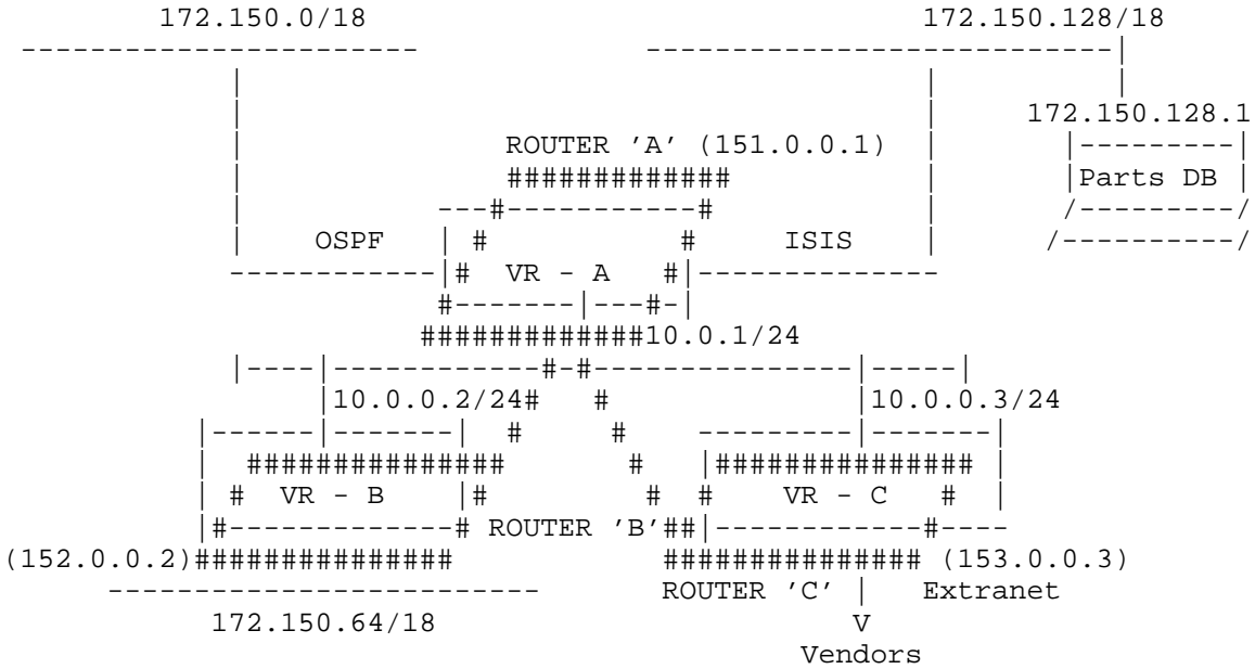
Figure 2 'Virtual Routing Domain'
