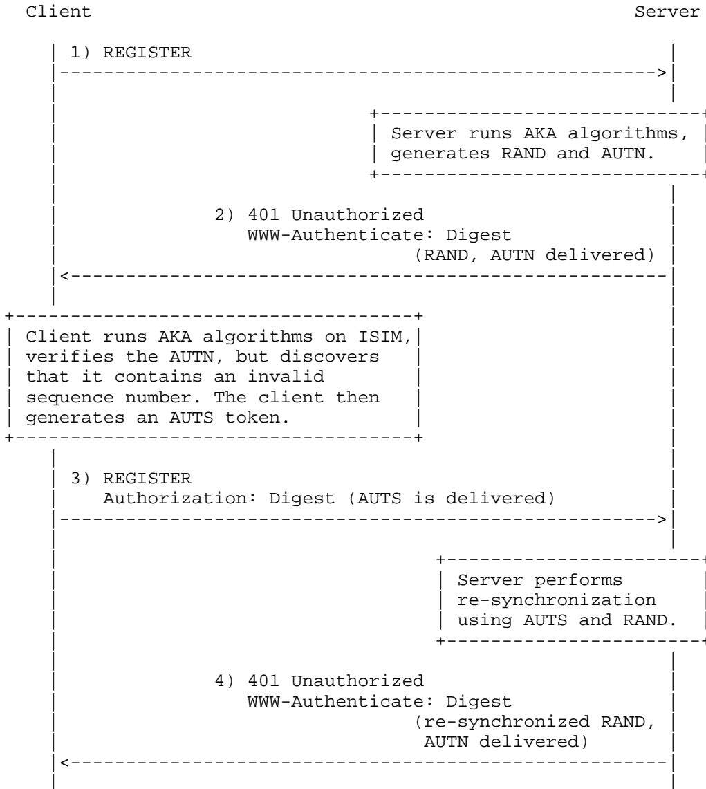
Figure 3: Message flow representing an authentication synchronization failure.
