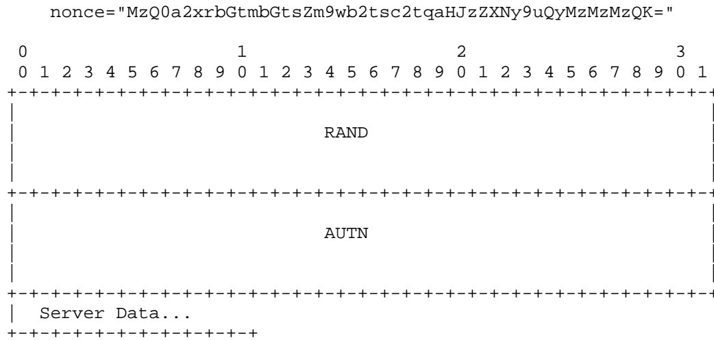
Figure 1: Generating the nonce value.
