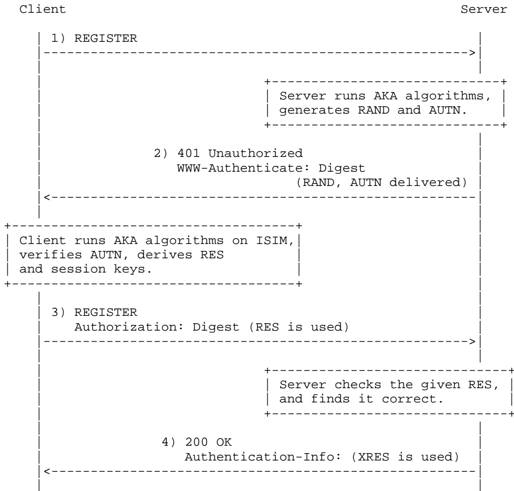
Figure 2: Message flow representing a successful authentication.
