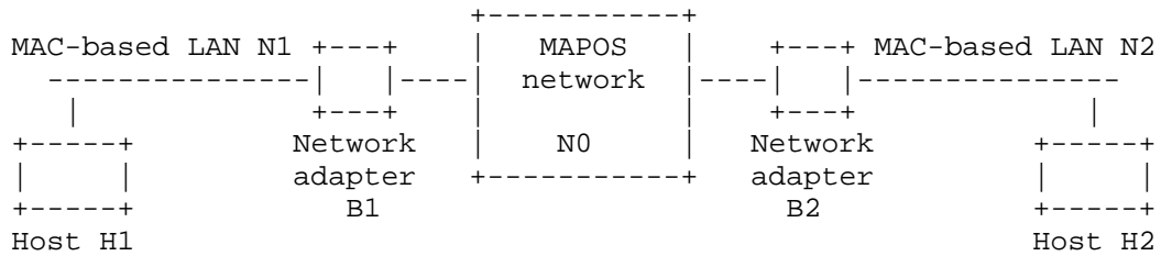
Figure 1. VPN network service model with LANs N1 and N2
