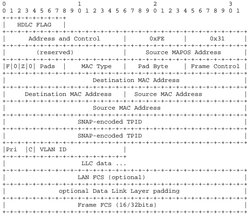
Figure 6. 802.4/802.5/FDDI Frame format (IEEE 802 Tagged Frame)
