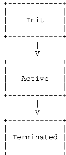
Figure 1: Registration State Machine
