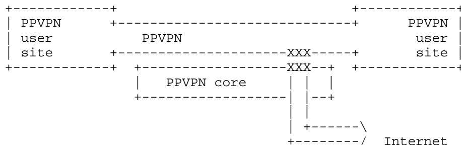
Figure 1: The PPVPN trusted zone model
