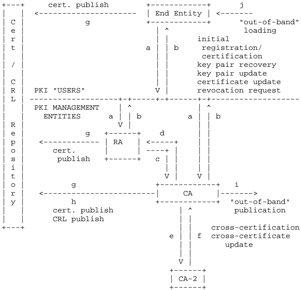
Figure 1 - PKI Entities
