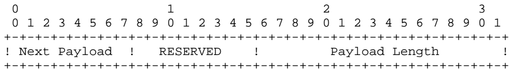
Figure 8: Generic Payload Header
