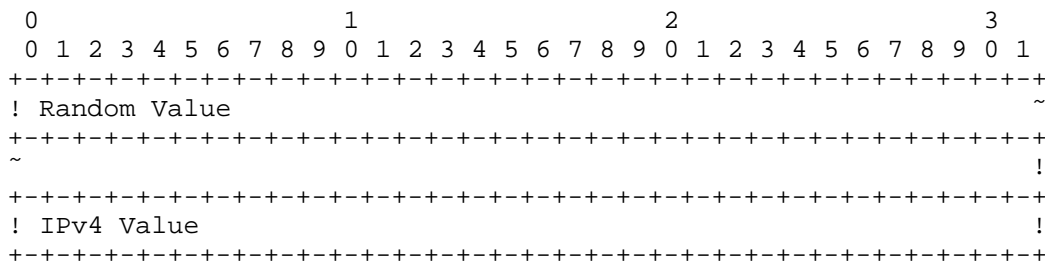
Figure 6: GroupID IPv4 Format
