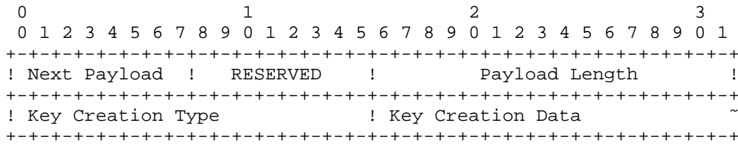
Figure 26: Key Creation Payload Format
