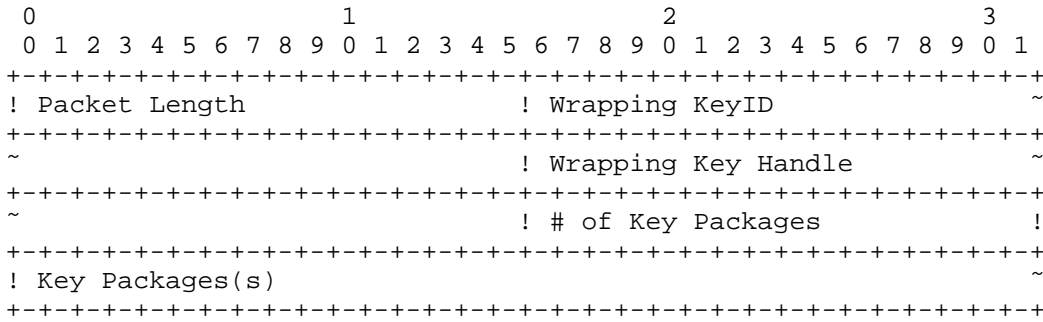
Figure 16: Rekey Event Data Format
