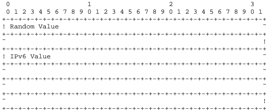
Figure 7: GroupID IPv6 Format
