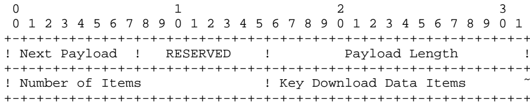
Figure 10: Key Download Payload Format
