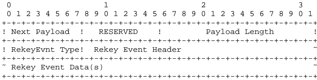
Figure 14: Rekey Event Payload Format
