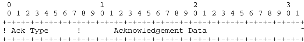
Figure 23: Notification Data - Acknowledge Payload Type Format
