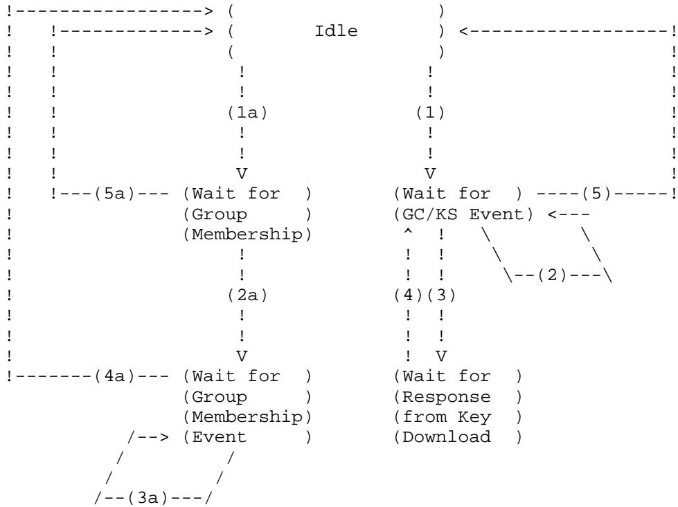
Figure 28: GSAKMP State Diagram
