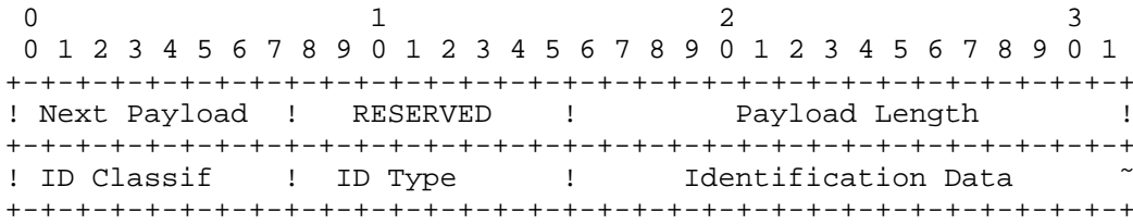
Figure 18: Identification Payload Format
