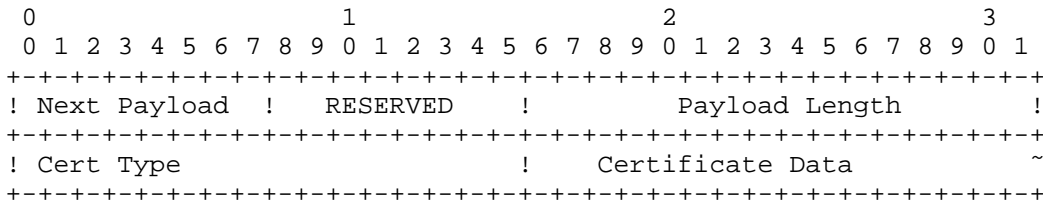
Figure 20: Certificate Payload Format
