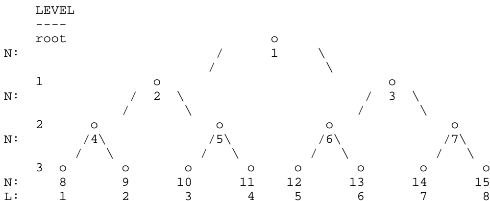
Figure 30: GSAKMP LKH Tree
