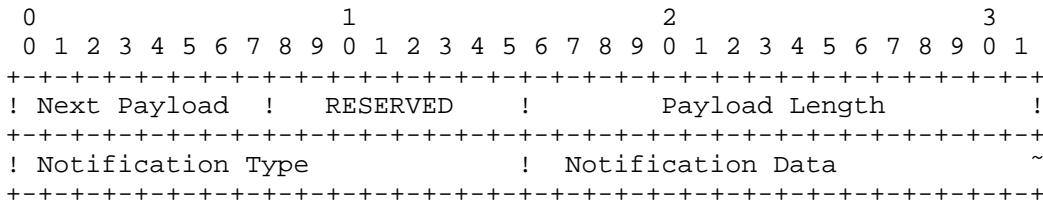
Figure 22: Notification Payload Format
