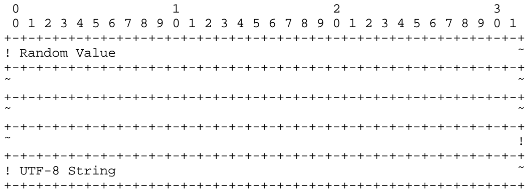
Figure 4: GroupID UTF-8 Format
