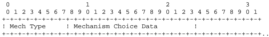
Figure 24: Notification Data - Mechanism Choices Payload Type Format
