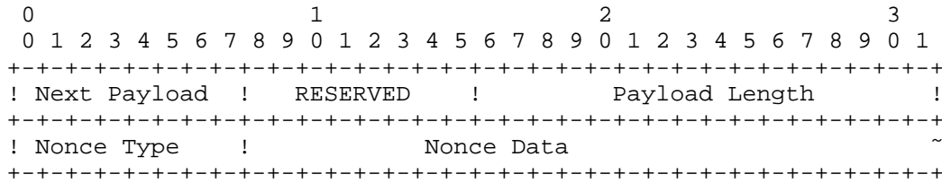
Figure 27: Nonce Payload Format
