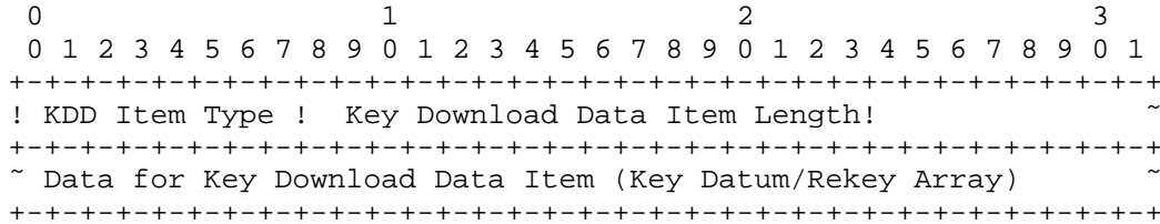
Figure 11: Key Download Data Item Format
