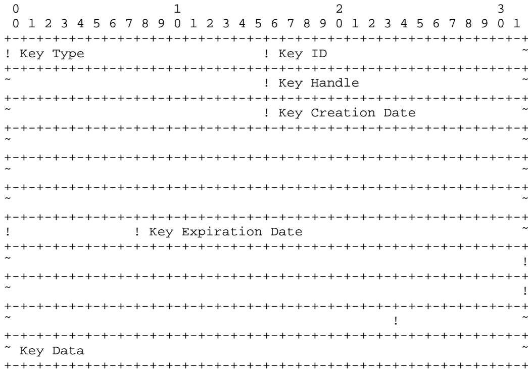
Figure 12: Key Datum Format
