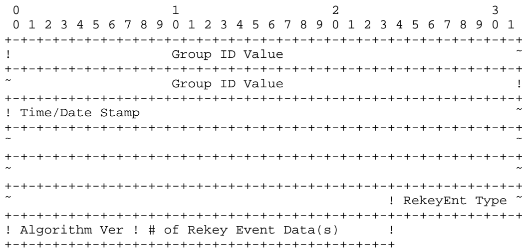
Figure 15: Rekey Event Header Format
