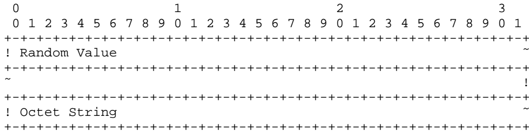
Figure 5: GroupID Octet String Format
