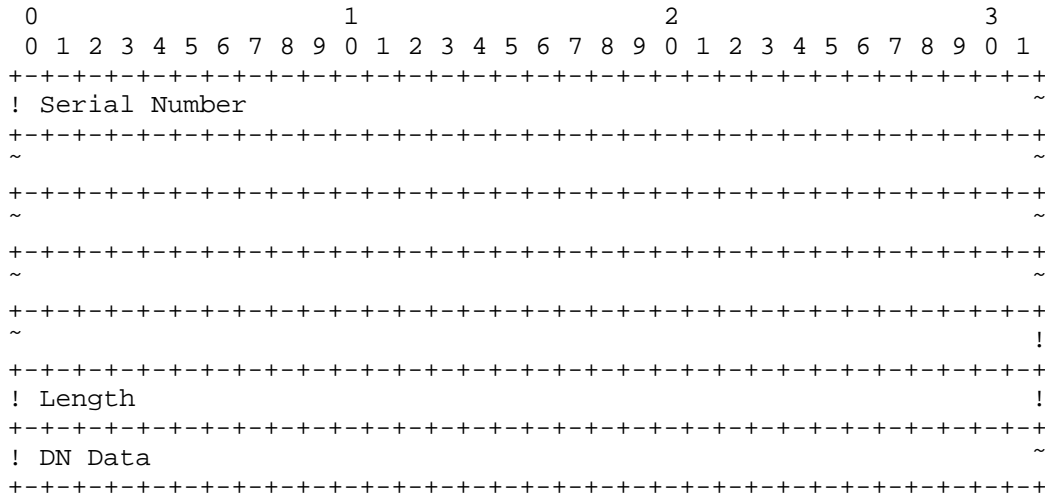
Figure 19: Unencoded Name (ID-U-NAME) Format
