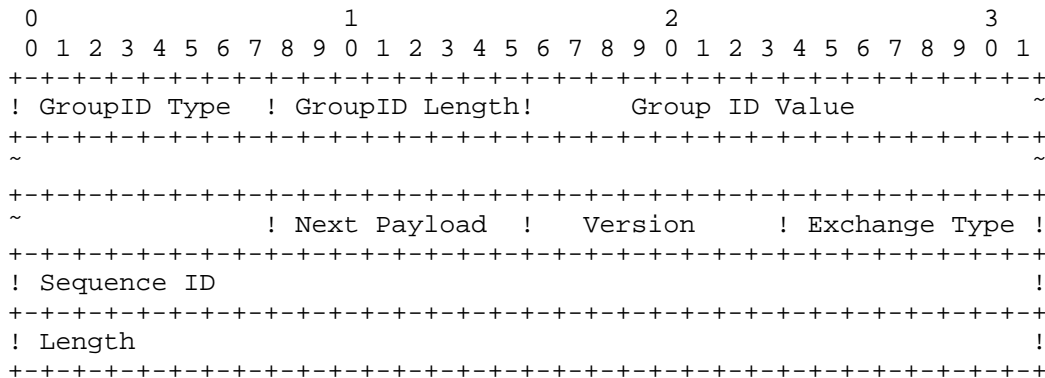
Figure 3: GSAKMP Header Format
