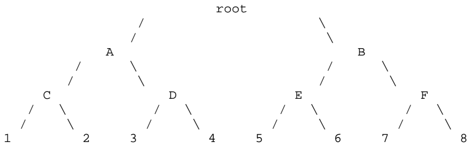
Figure 29: LKH Tree
