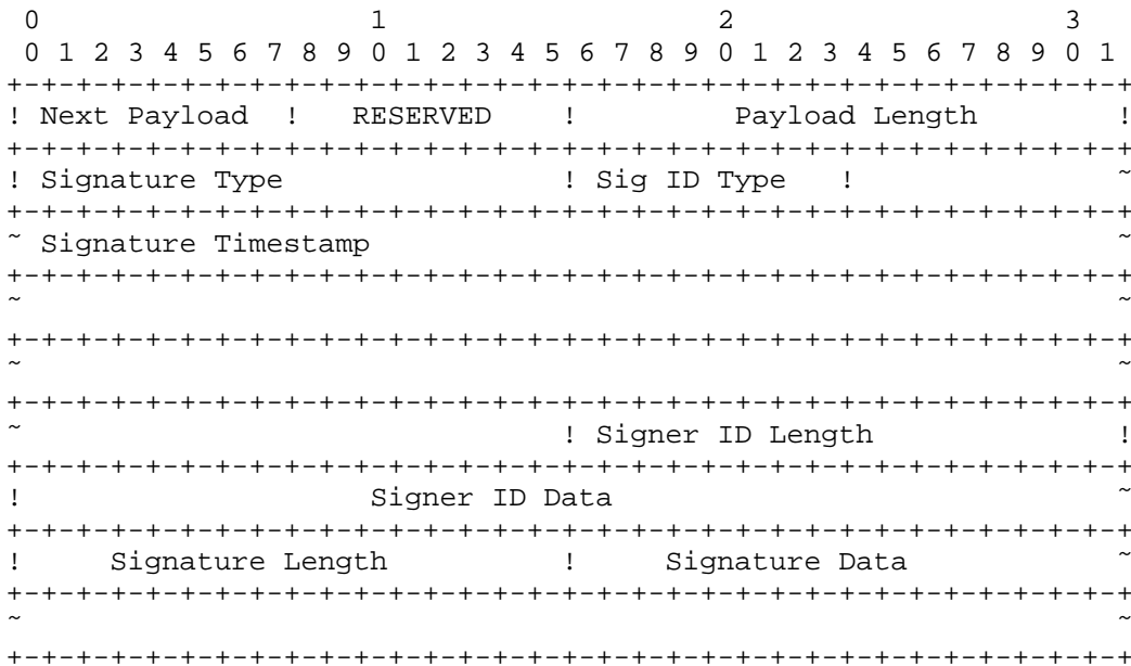
Figure 21: Signature Payload Format
