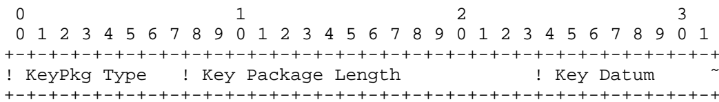
Figure 17: Key Package Format
