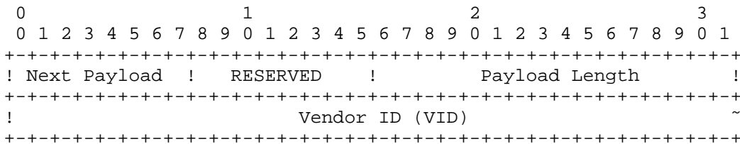
Figure 25: Vendor ID Payload Format
