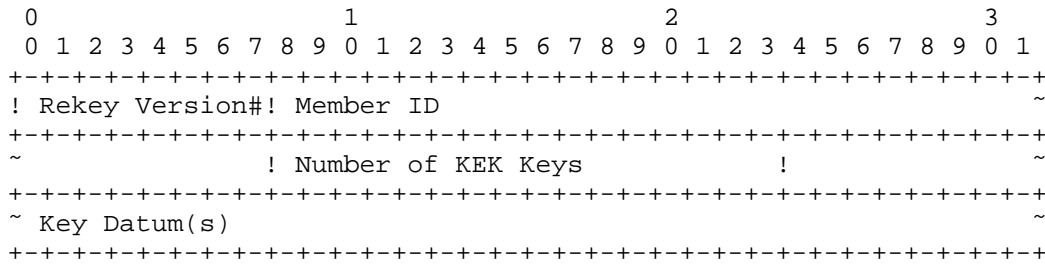
Figure 13: Rekey Array Structure Format
