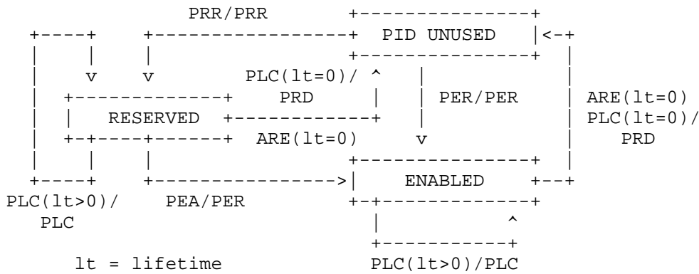
Figure 42: Policy rule state machine
