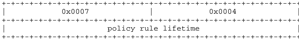
Figure 10: Policy rule lifetime attribute
