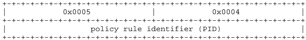
Figure 8: Policy rule identifier attribute
