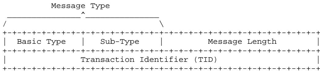
Figure 2: The SIMCO header
