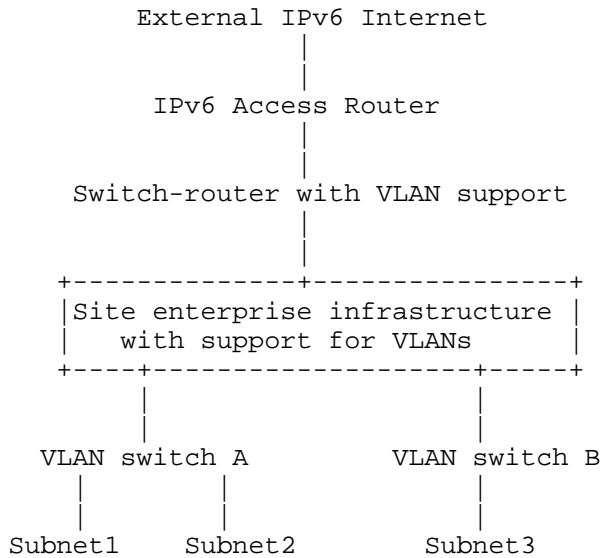
Figure 1: IPv6 deployment using VLANs (physical diagram)
