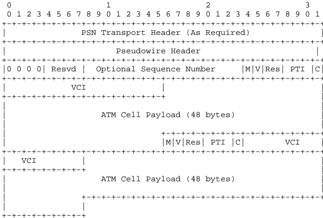
Figure 10: Multiple Cell VPC Encapsulation
