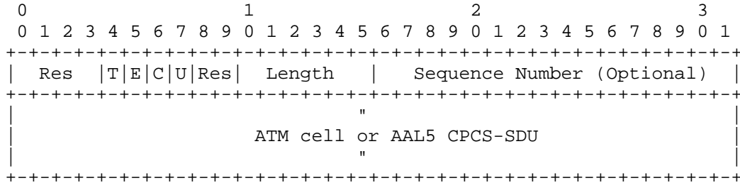
Figure 11: AAL5 CPCS-SDU Encapsulation
