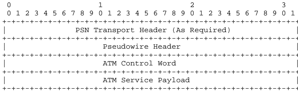
Figure 2: General format for ATM encapsulation over PSNs
