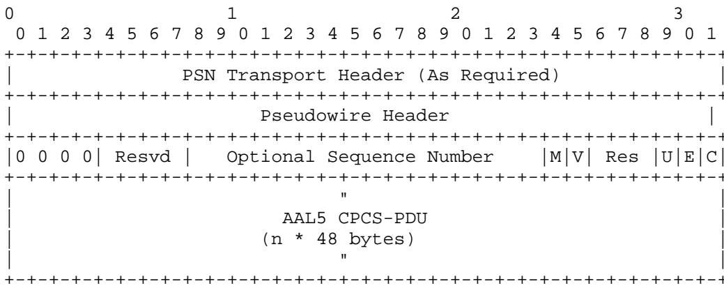
Figure 12: AAL5 transparent service encapsulation
