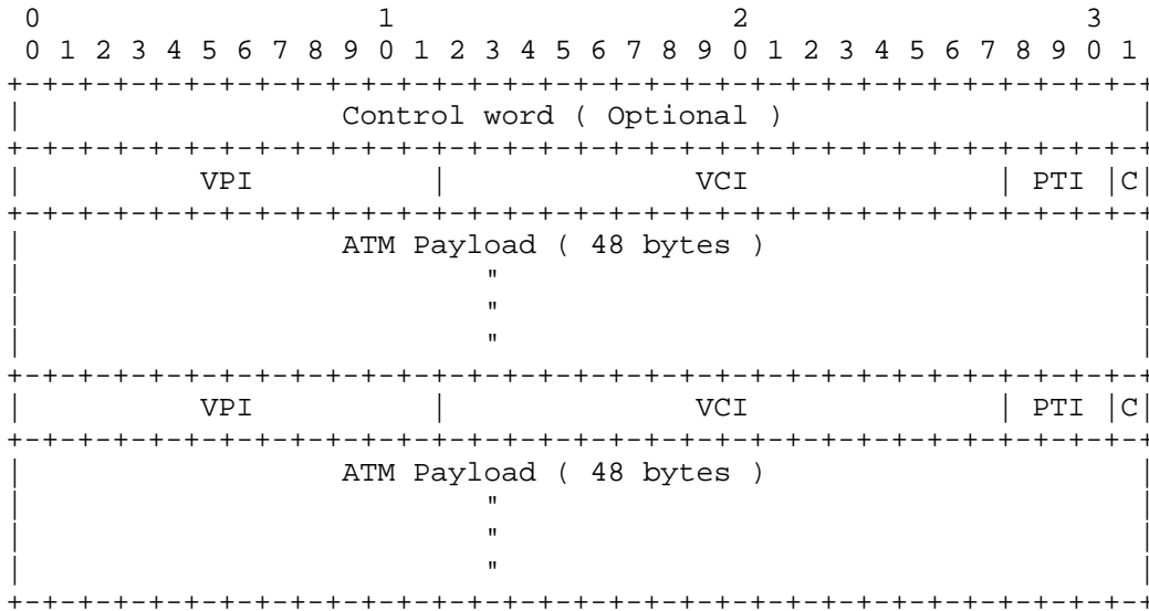
Figure 5: Multiple Cell ATM Encapsulation
