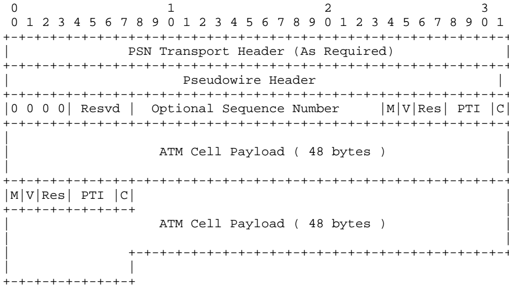
Figure 8: Multiple ATM VCC Cell Encapsulation
