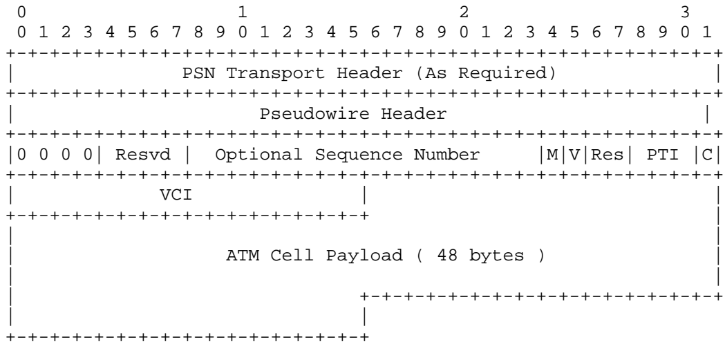
Figure 9: Single Cell VPC Encapsulation
