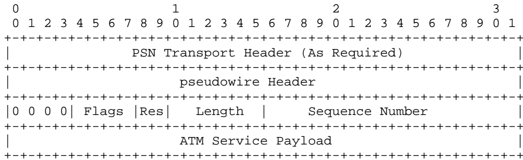
Figure 4: General format for ATM encapsulation over PSNs
