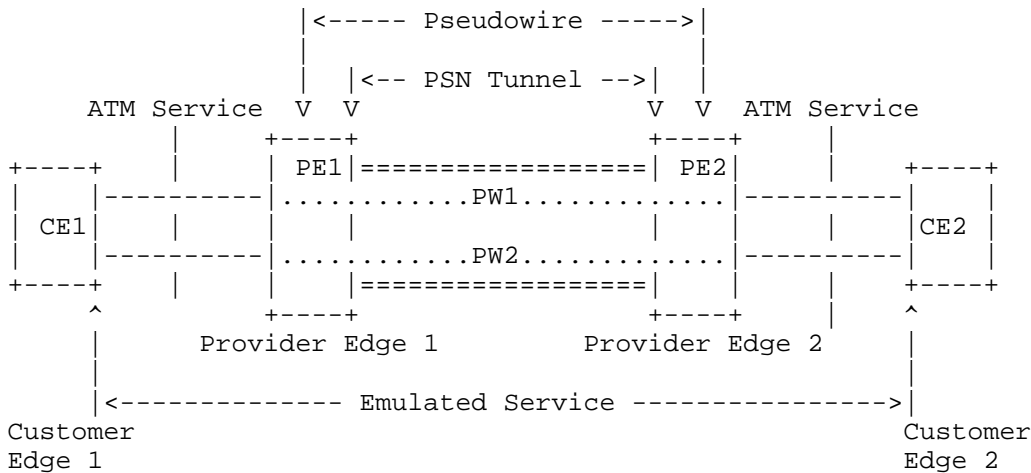
Figure 1: ATM Service Reference Model
