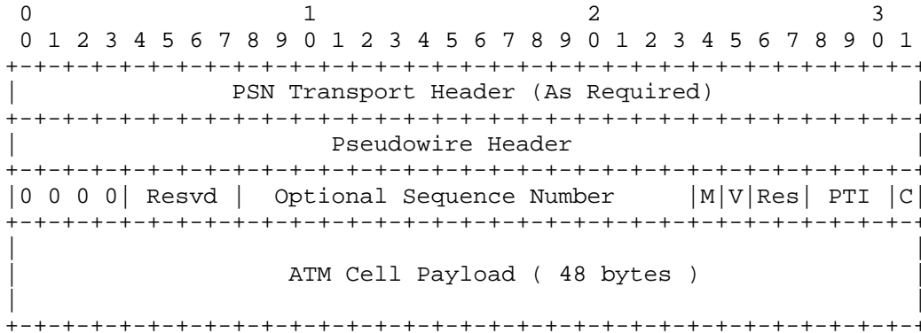
Figure 7: Single ATM VCC Cell Encapsulation
