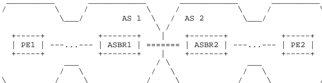
Figure 5: Inter-AS VPLS
