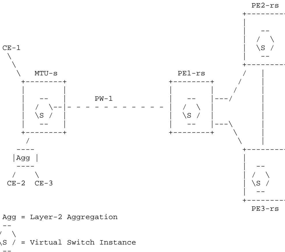
Figure 3: An example of a hierarchical VPLS model
