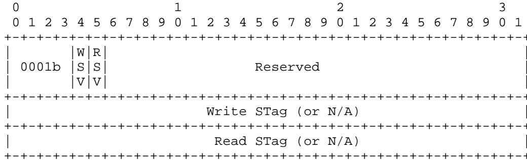
Figure 3. iSER Header Format for iSCSI Control-Type PDU
