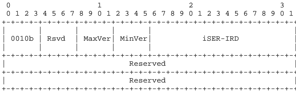
Figure 4. iSER Header Format for iSER Hello Message
