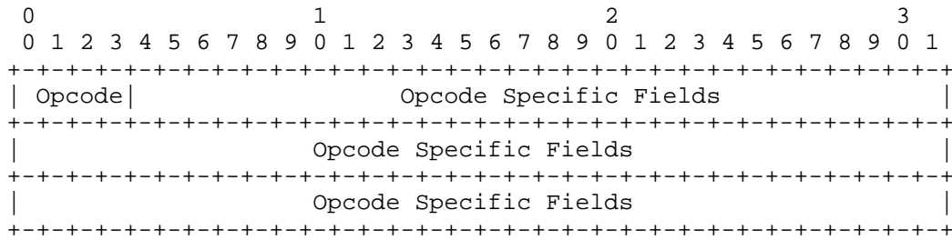
Figure 2. iSER Header Format
