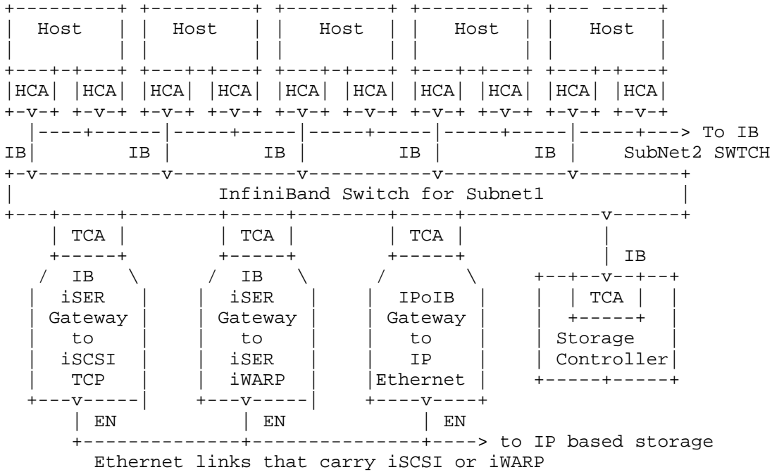
Figure 14. iSCSI and iSER on IB
