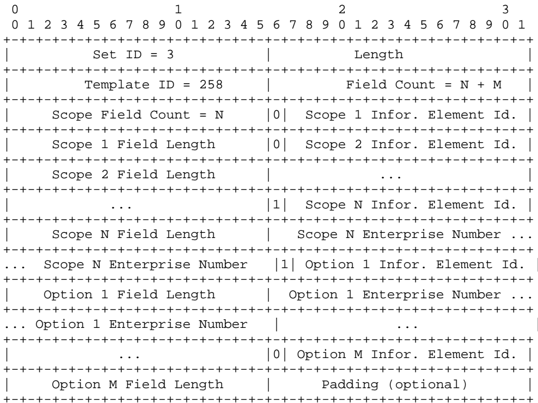
Figure 0: Option Template Set Example
