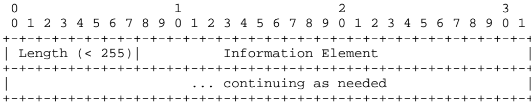
Figure R: Variable-Length Information Element (length < 255 octets)
