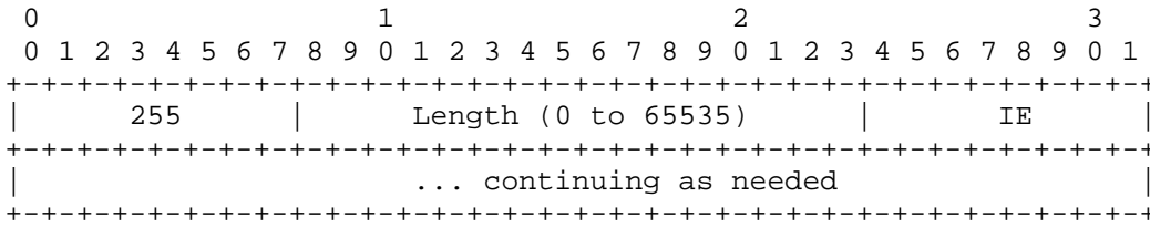
Figure S: Variable-Length Information Element (length 0 to 65535 octets)
