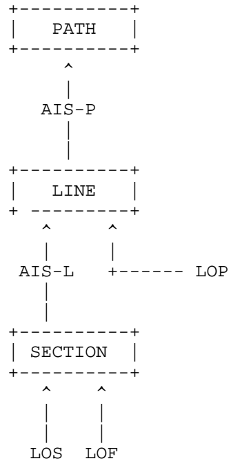
Figure 6. SONET/SDH Fault Hierarchy
