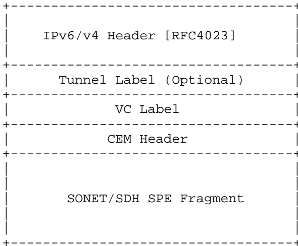
Figure 4. MPLS Transport Encapsulation
