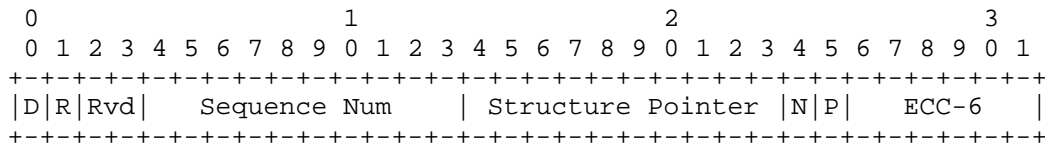
Figure 2. CEM Header Format
