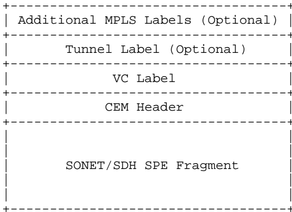
Figure 3. Typical MPLS Transport Encapsulation
