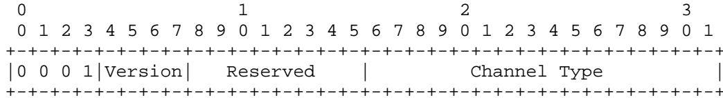
Figure 1: Associated Channel Header
