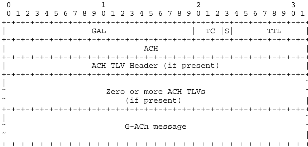
Figure 8: G-ACh Packet Format for an MPLS Section
