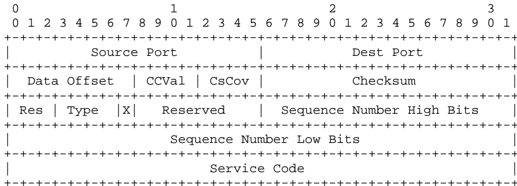
Figure 1: Format of a DCCP-Listen Packet
