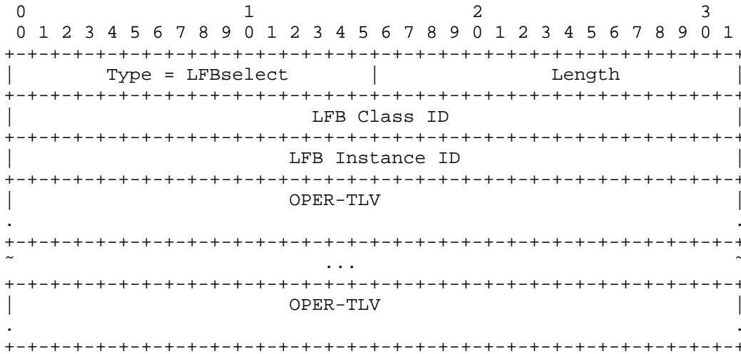
Figure 19: PL PDU Layout
