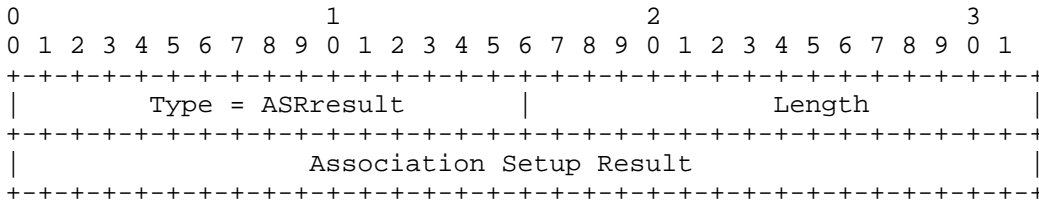
Figure 25: ASResult OPER-TLV
