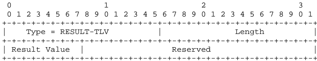
Figure 20: RESULT-TLV
