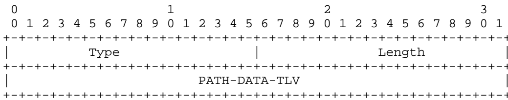
Figure 29: OPER-TLV for Config
