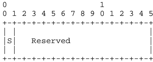
Figure 18: Path Flags
