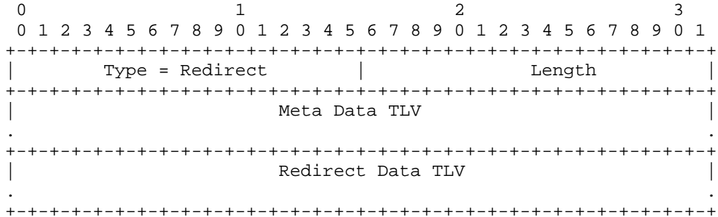
Figure 39: Redirect_Data TLV
