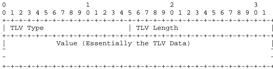
Figure 14: TLV Representation
