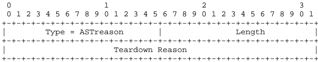
Figure 27: ASTreason-TLV
