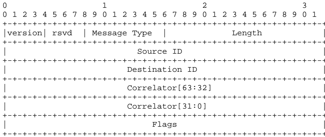
Figure 10: Common Header
