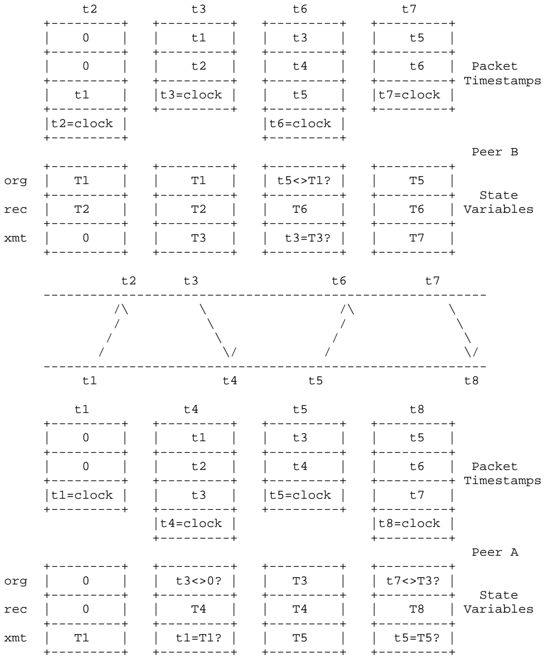
Figure 15: On-Wire Protocol
