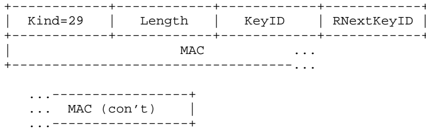
Figure 2: The TCP Authentication Option (TCP-AO)
